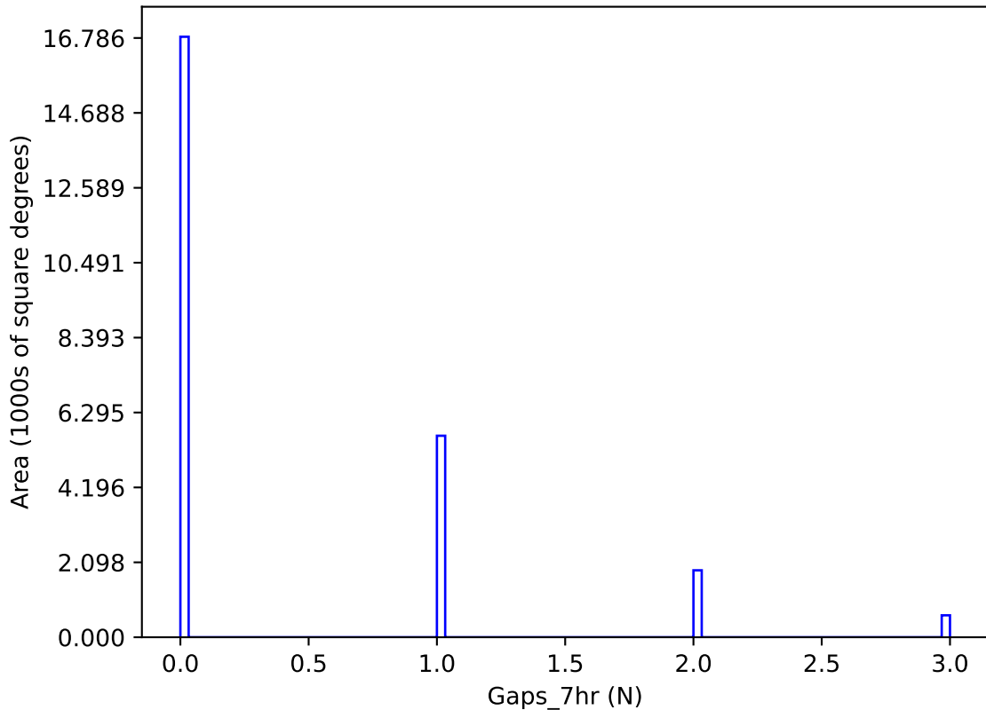
ddf_loaded_fl8_v3.4_10yrs y band: Gaps_7hr
