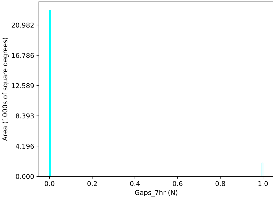
ddf_loaded_fl8_v3.4_10yrs u band: Gaps_7hr
