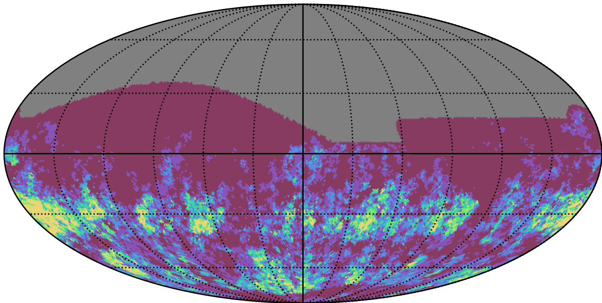
ddf_loaded_fl8_v3.4_10yrs r band: Gaps_7hr
