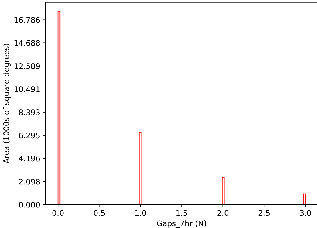
ddf_loaded_fl8_v3.4_10yrs i band: Gaps_7hr
