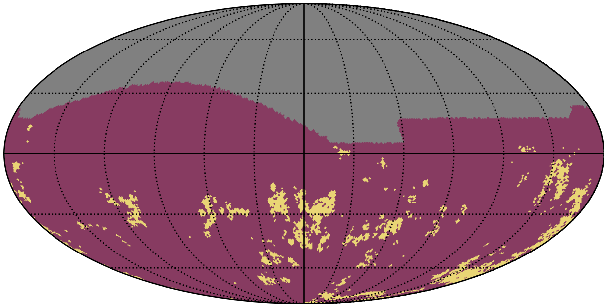
ddf_loaded_fl8_v3.4_10yrs g band: Gaps_7hr
