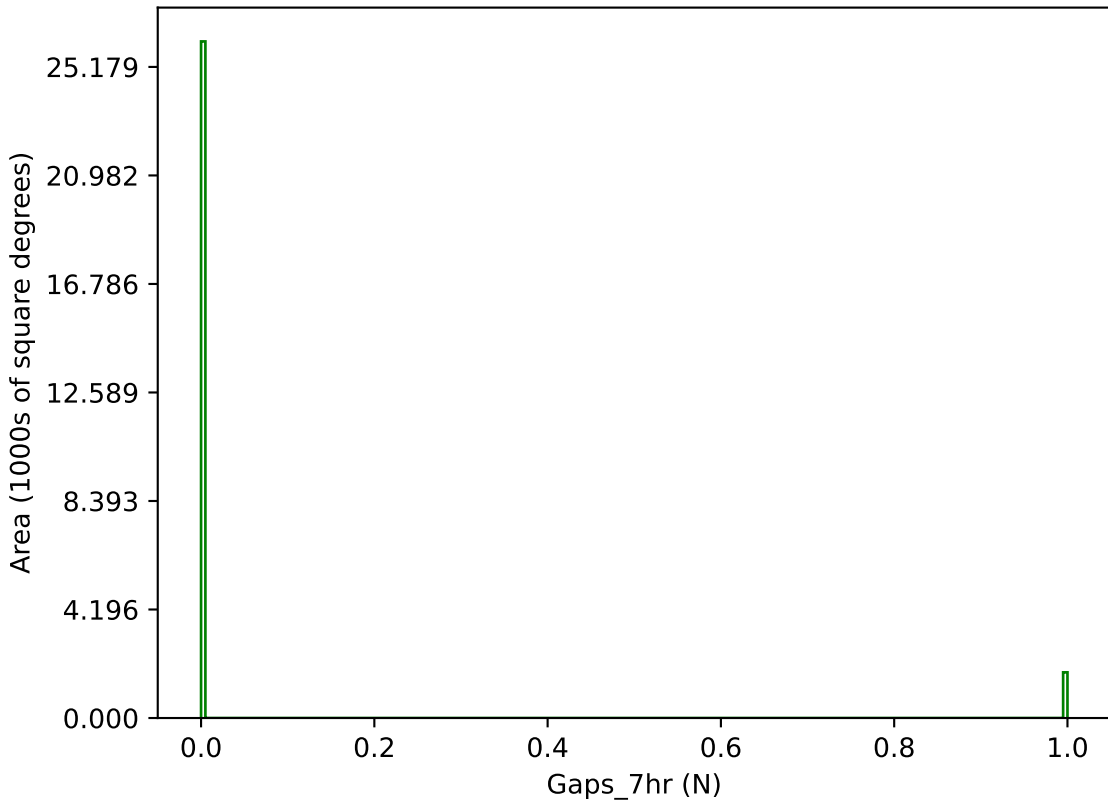
ddf_loaded_fl8_v3.4_10yrs g band: Gaps_7hr
