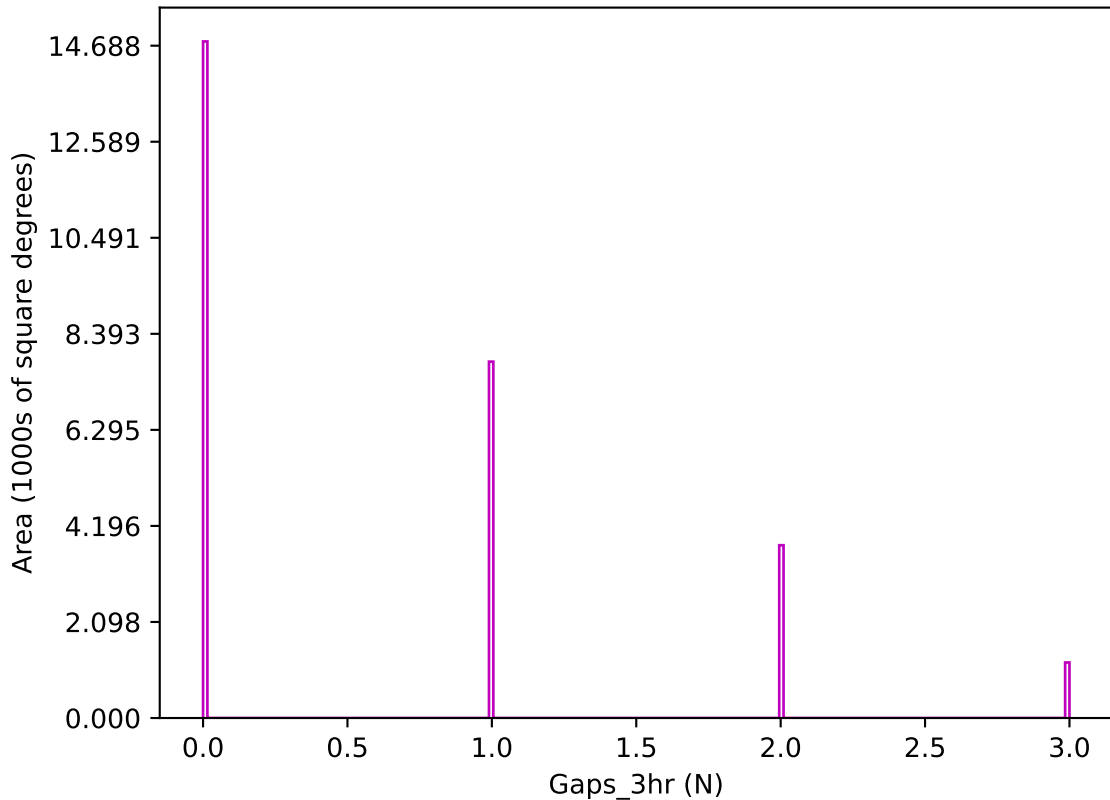
ddf_loaded_fl8_v3.4_10yrs z band: Gaps_3hr
