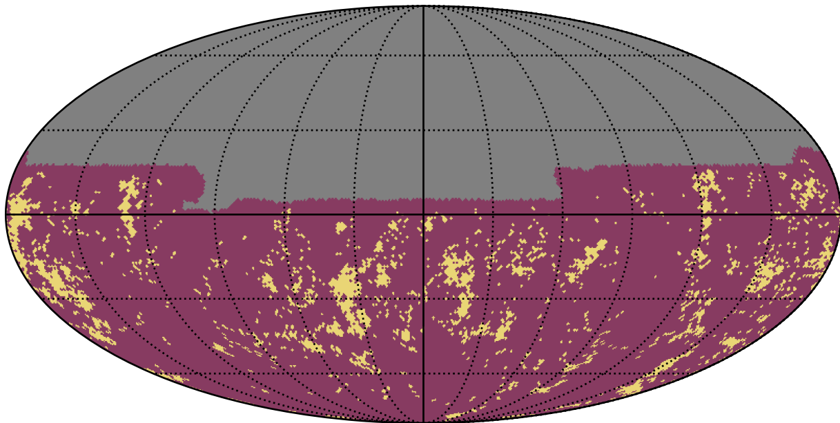
ddf_loaded_fl8_v3.4_10yrs u band: Gaps_3hr
