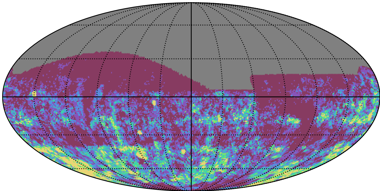
ddf_loaded_fl8_v3.4_10yrs r band: Gaps_3hr
