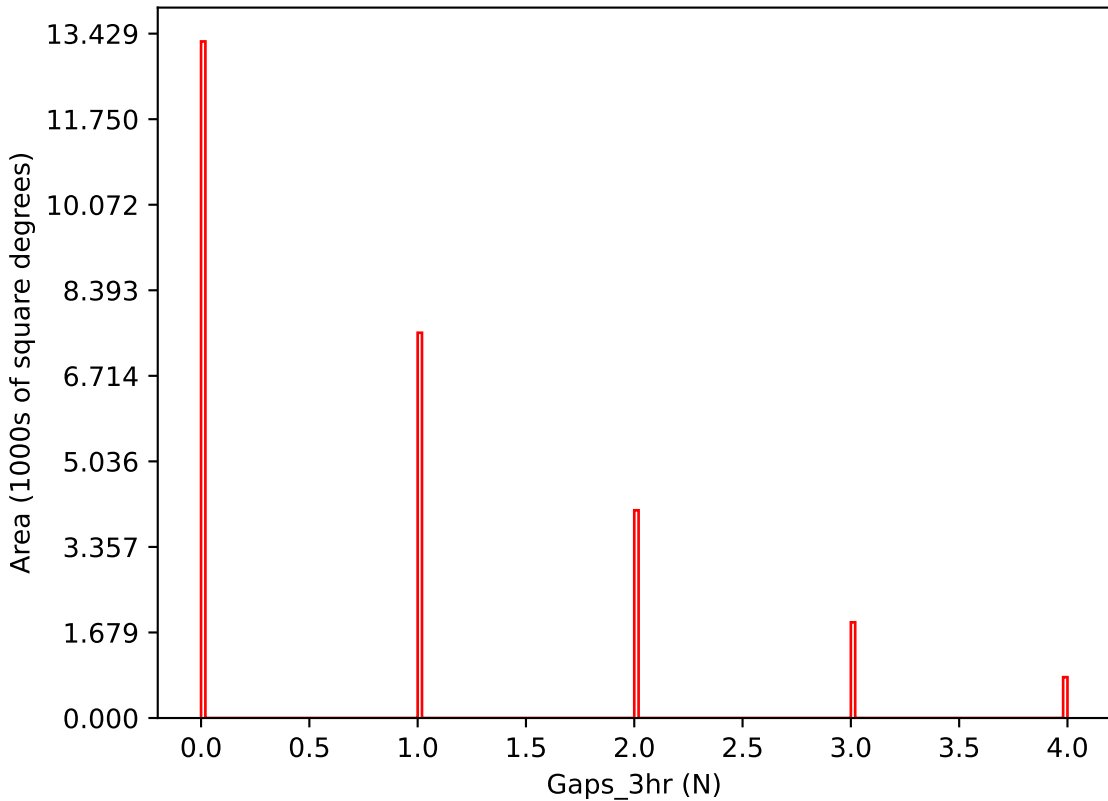
ddf_loaded_fl8_v3.4_10yrs i band: Gaps_3hr
