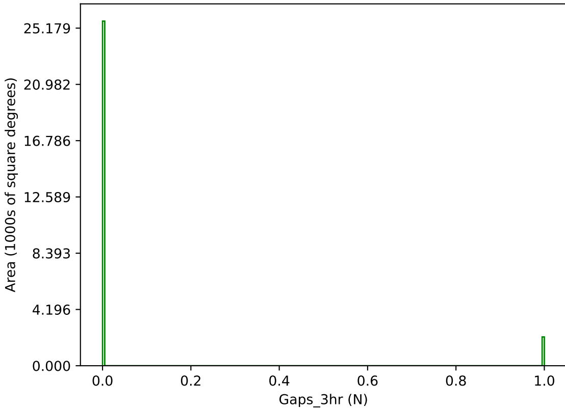
ddf_loaded_fl8_v3.4_10yrs g band: Gaps_3hr
