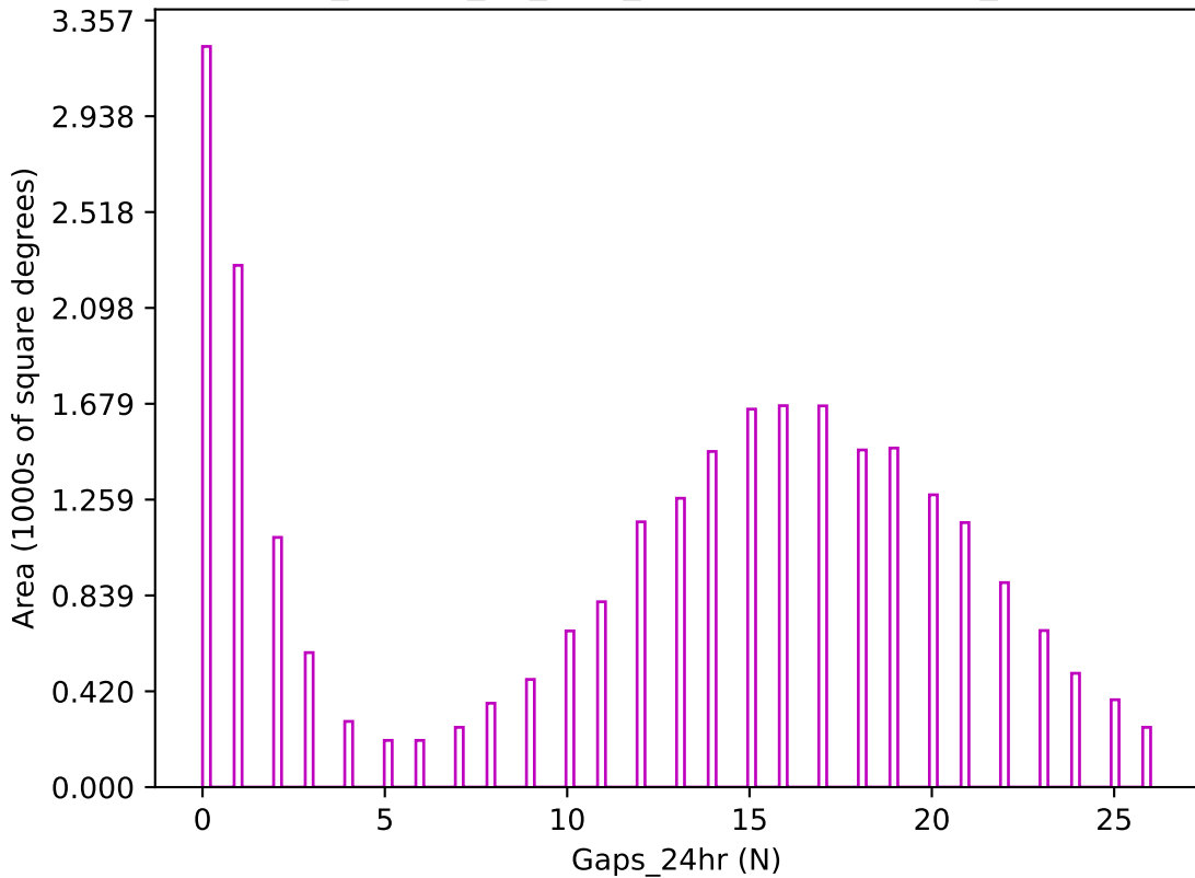
ddf_loaded_fl8_v3.4_10yrs z band: Gaps_24hr
