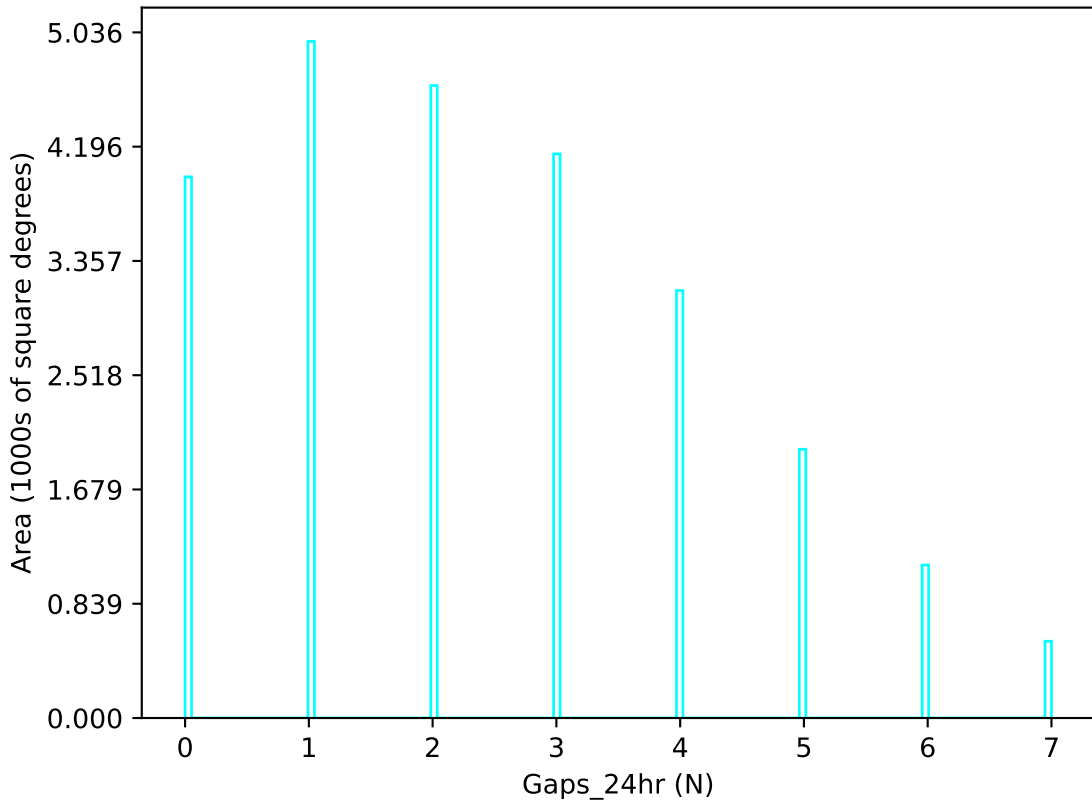
ddf_loaded_fl8_v3.4_10yrs u band: Gaps_24hr
