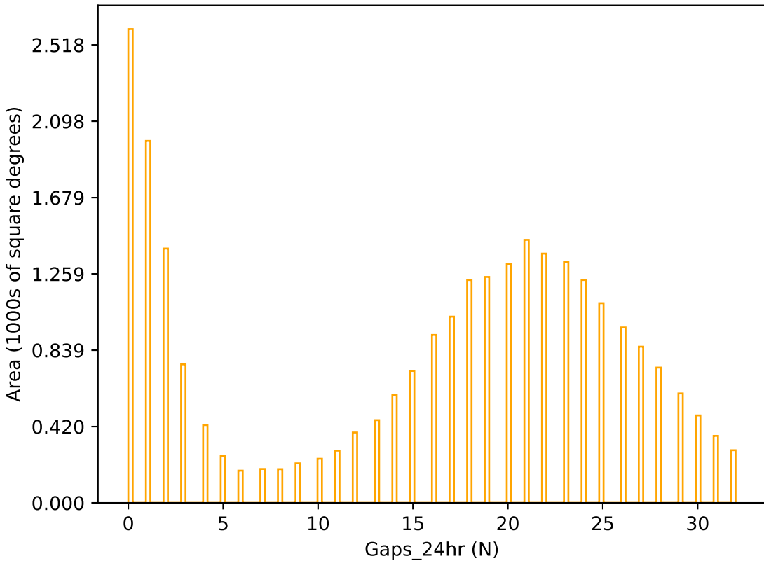
ddf_loaded_fl8_v3.4_10yrs r band: Gaps_24hr
