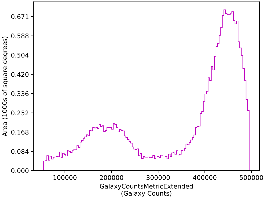
ddf_loaded_fl8_v3.4_10yrs z: GalaxyCountsMetricExtended
