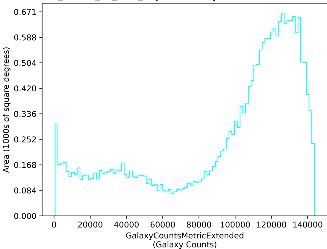
ddf_loaded_fl8_v3.4_10yrs u: GalaxyCountsMetricExtended
