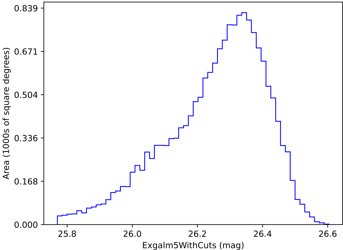
ddf_loaded_fl8_v3.4_10yrs i band non-DD year 8: ExgalM5WithCuts
