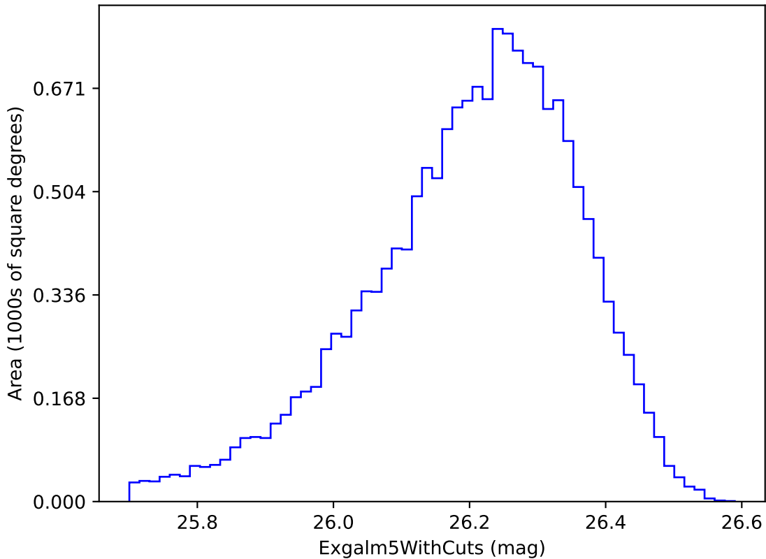
ddf_loaded_fl8_v3.4_10yrs i band non-DD year 7: Exgal5WithCuts
