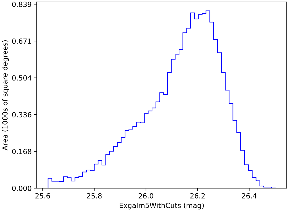
ddf_loaded_fl8_v3.4_10yrs i band non-DD year 6: ExgalM5WithCuts
