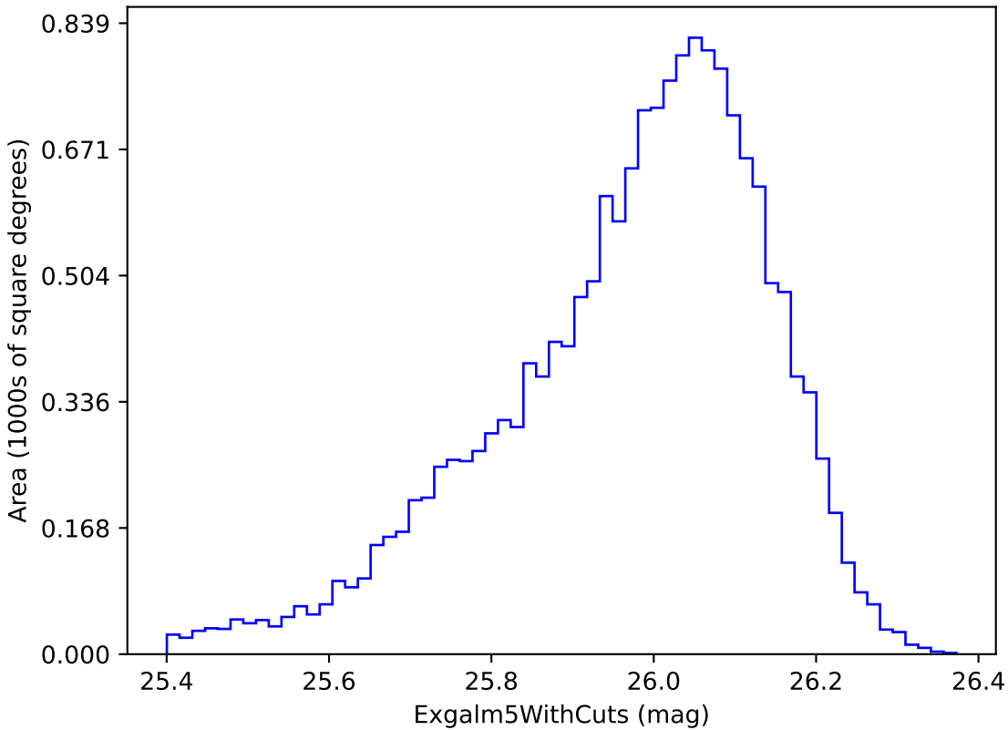
ddf_loaded_fl8_v3.4_10yrs i band non-DD year 4: ExgalM5WithCuts
