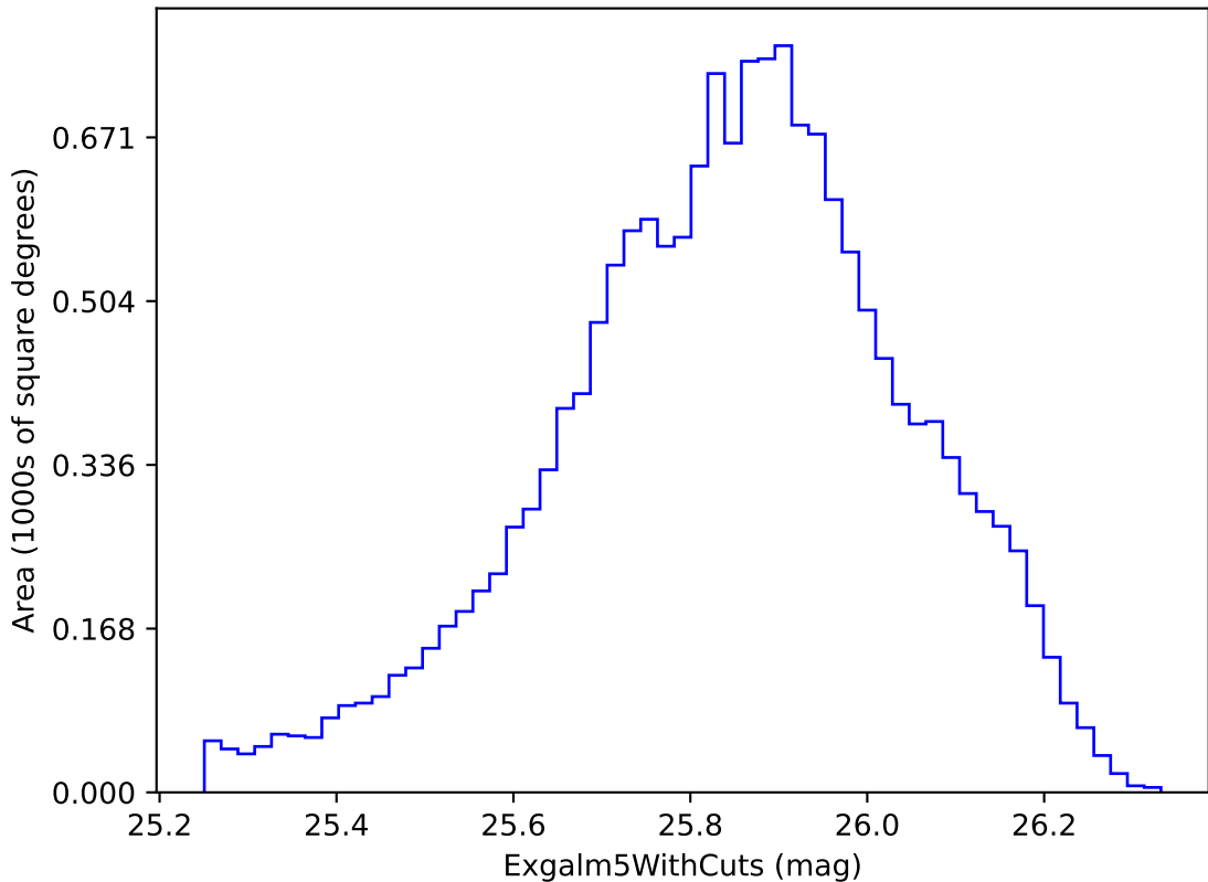
ddf_loaded_fl8_v3.4_10yrs i band non-DD year 3: ExgalM5WithCuts
