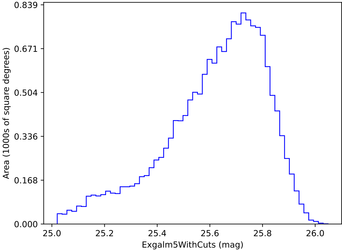
ddf_loaded_fl8_v3.4_10yrs i band non-DD year 2: ExgalM5WithCuts
