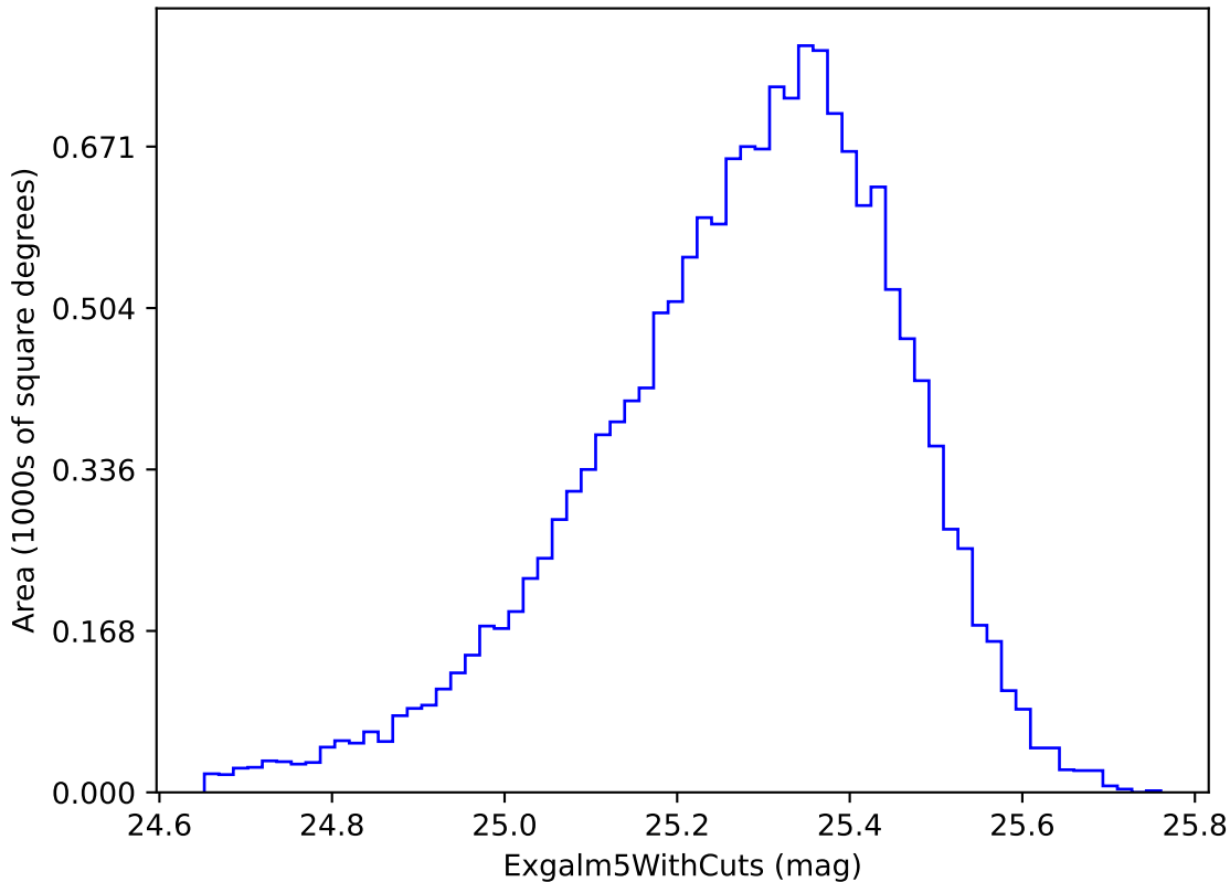
ddf_loaded_fl8_v3.4_10yrs i band non-DD year 1: ExgalM5WithCuts
