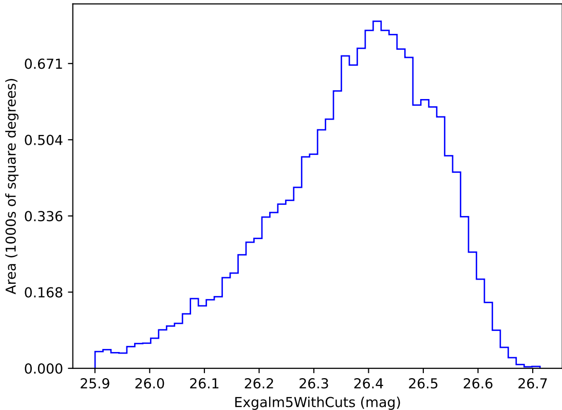
ddf_loaded_fl8_v3.4_10yrs i band non-DD year 10: ExgalM5WithCuts
