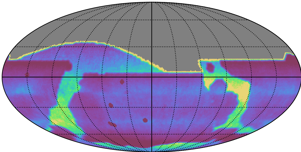
ddf_loaded_fl8_v3.4_10yrs : DCRprecision
