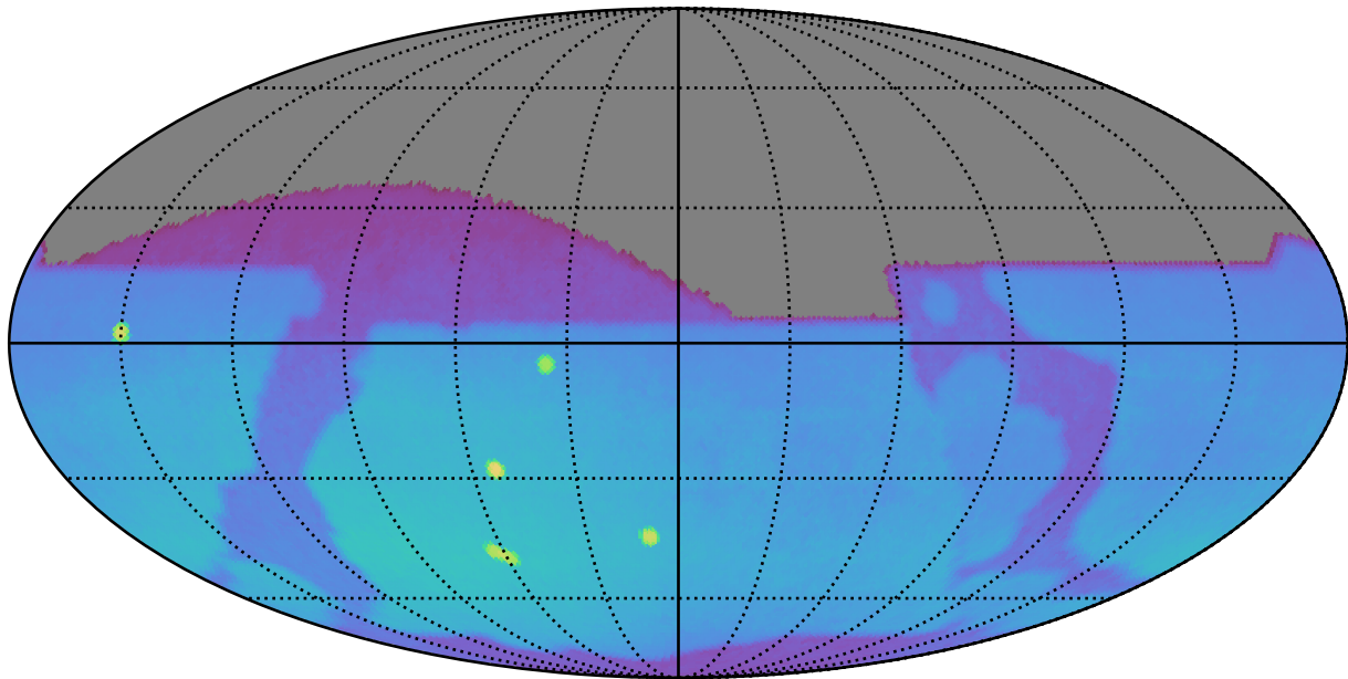
ddf_loaded_fl8_v3.4_10yrs : Brown Dwarf, L7
