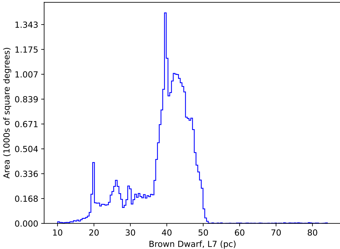
ddf_loaded_fl8_v3.4_10yrs : Brown Dwarf, L7
