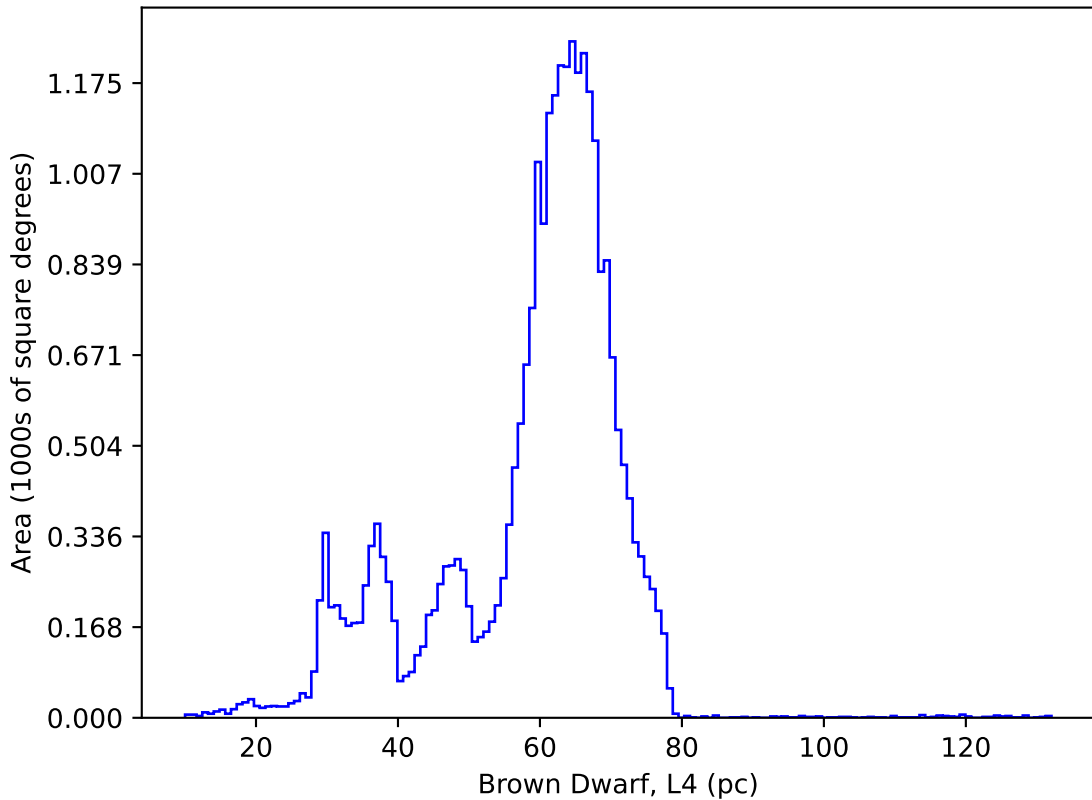
ddf_loaded_fl8_v3.4_10yrs : Brown Dwarf, L4
