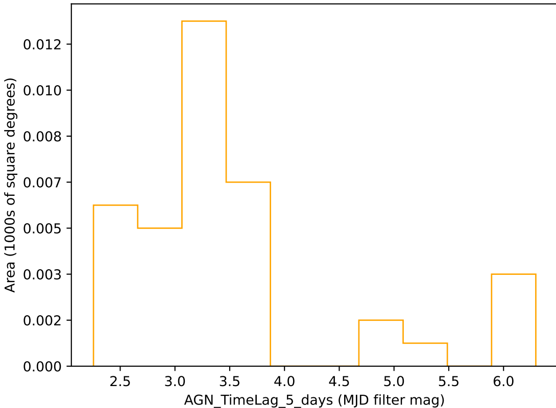
ddf_loaded_fl8_v3.4_10yrs r band: AGN_TimeLag_5_days
