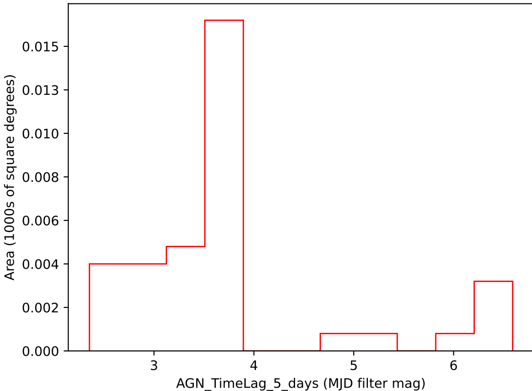
ddf_loaded_fl8_v3.4_10yrs i band: AGN_TimeLag_5_days
