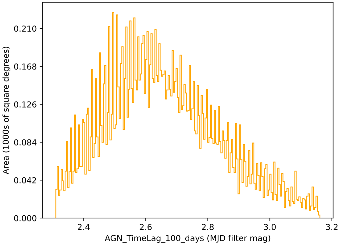
ddf_loaded_fl8_v3.4_10yrs r band: AGN_TimeLag_100_days
