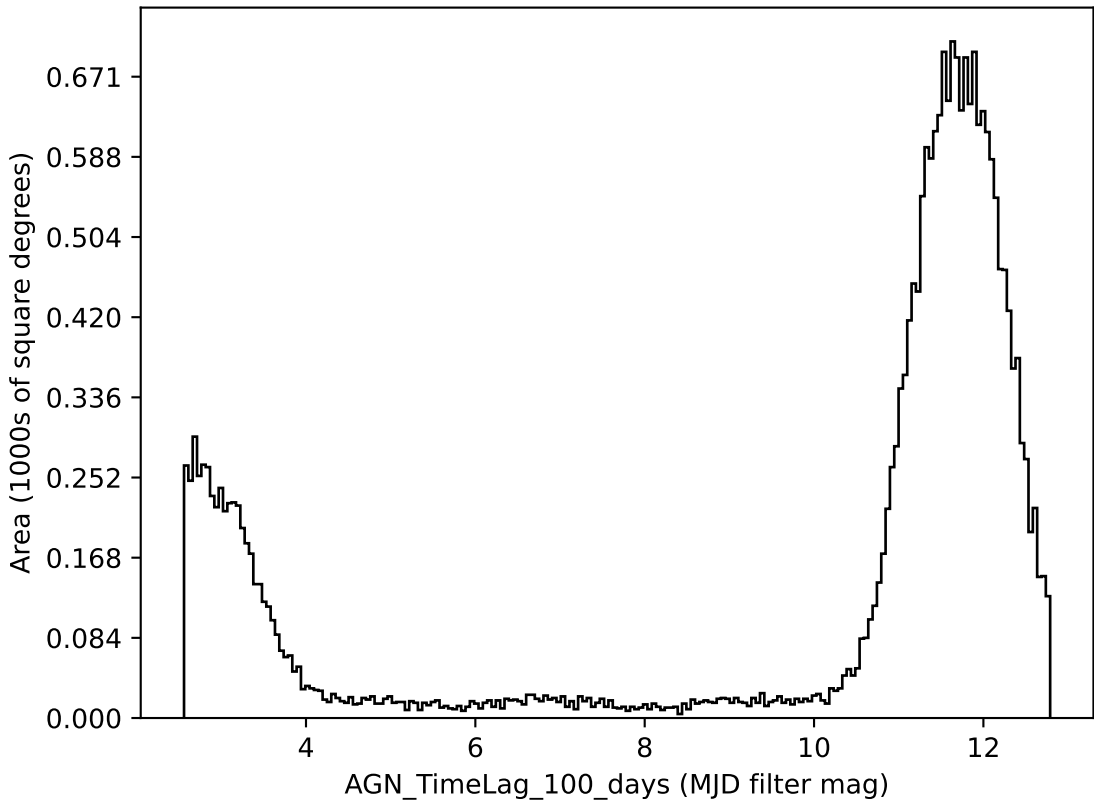
ddf_loaded_fl8_v3.4_10yrs all bands: AGN_TimeLag_100_days
