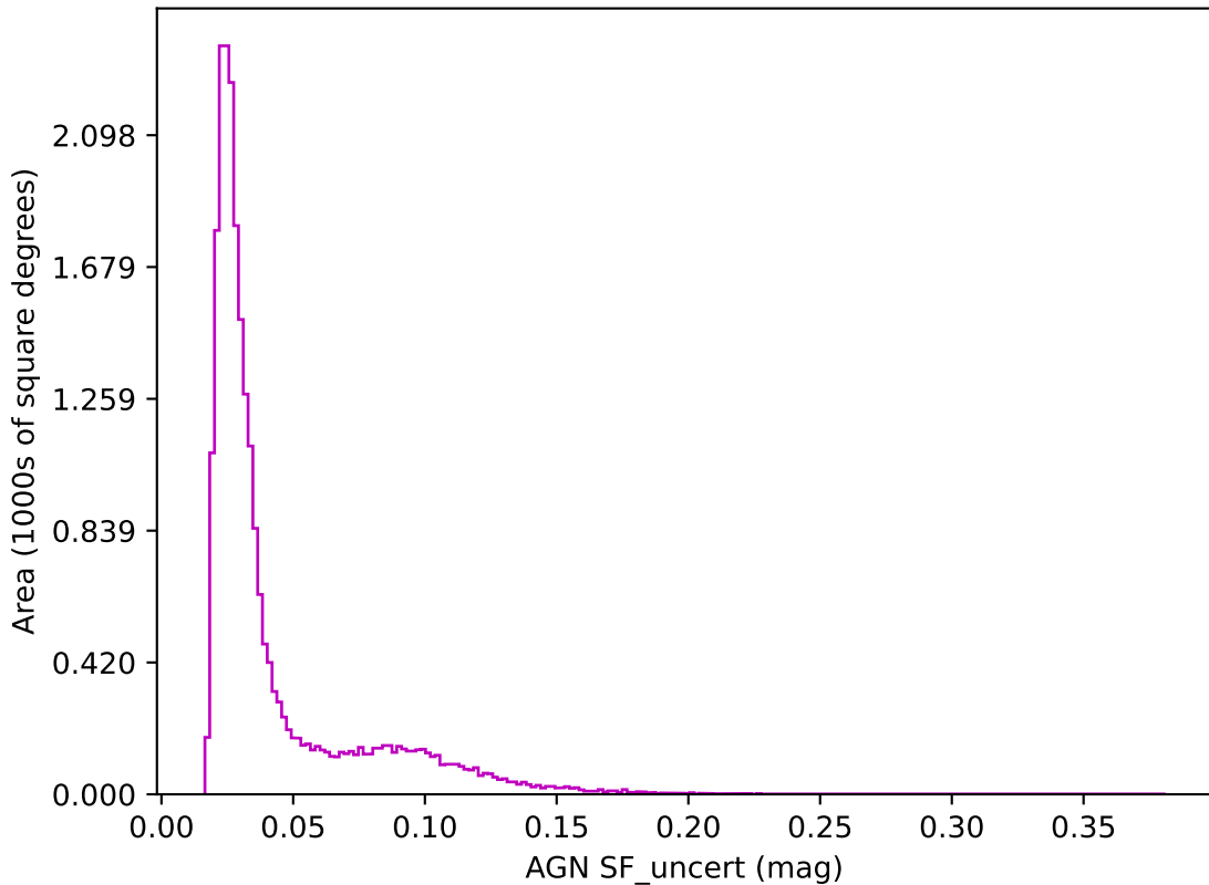
ddf_loaded_fl8_v3.4_10yrs z band: AGN SF_uncert
