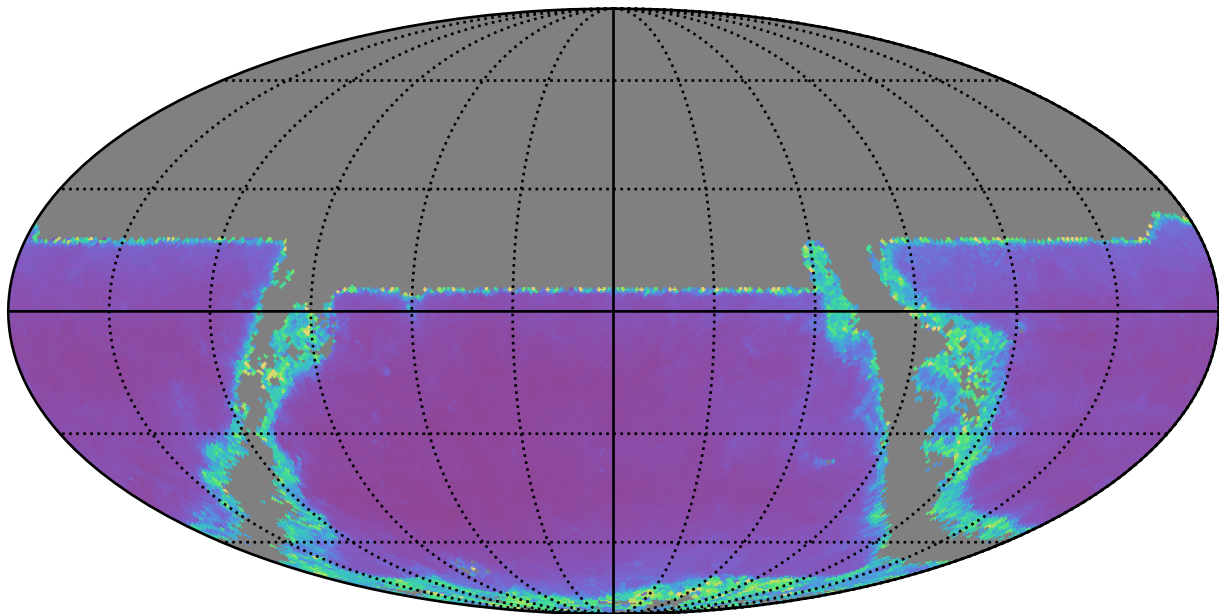
ddf_loaded_fl8_v3.4_10yrs y band: AGN SF_uncert
