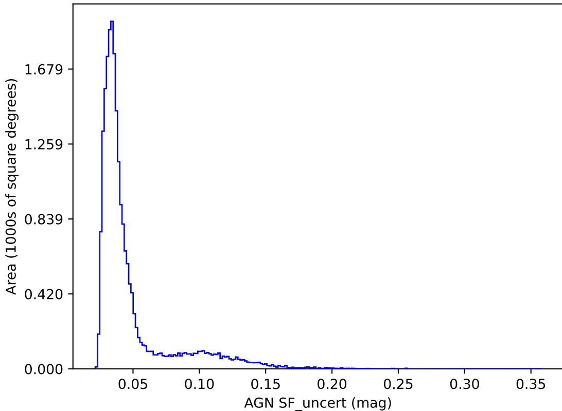
ddf_loaded_fl8_v3.4_10yrs y band: AGN SF_uncert
