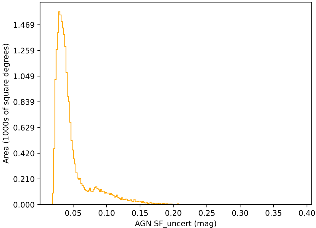
ddf_loaded_fl8_v3.4_10yrs r band: AGN SF_uncert
