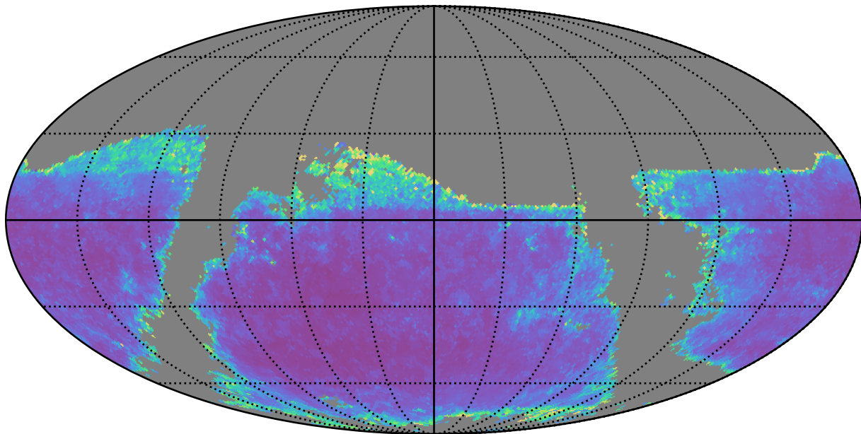
ddf_loaded_fl8_v3.4_10yrs g band: AGN SF_uncert
