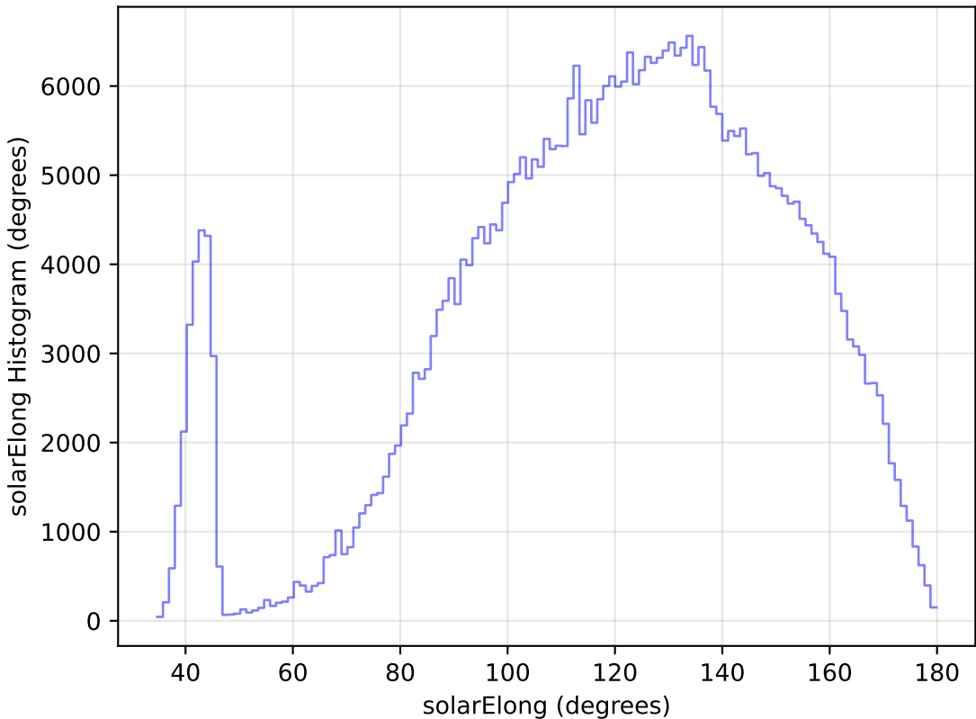
ddf_loaded_fl8_v3.4_10yrs WFD z band: solarElong Histogram
