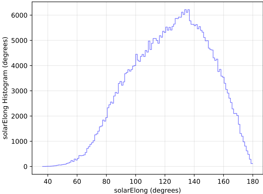
ddf_loaded_fl8_v3.4_10yrs WFD y band: solarElong Histogram
