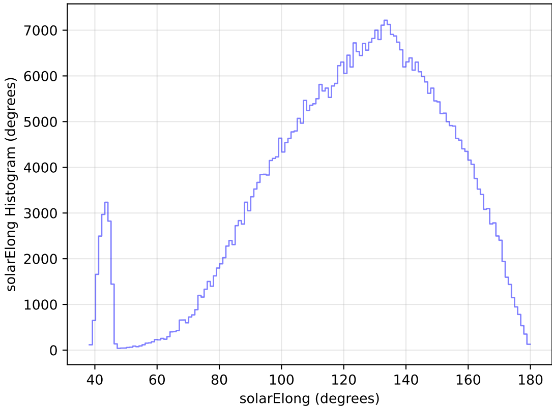
ddf_loaded_fl8_v3.4_10yrs WFD r band: solarElong Histogram
