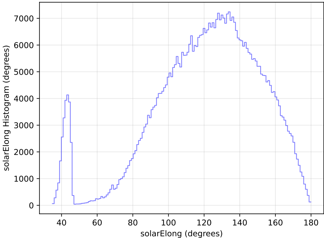
ddf_loaded_fl8_v3.4_10yrs WFD i band: solarElong Histogram
