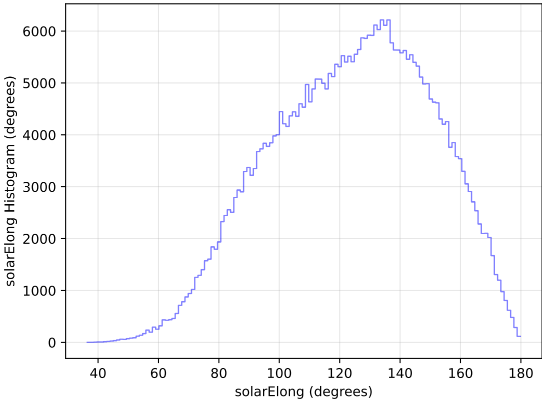
ddf_loaded_fl8_v3.4_10yrs All sky y band: solarElong Histogram
