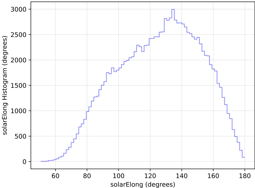
ddf_loaded_fl8_v3.4_10yrs All sky u band: solarElong Histogram
