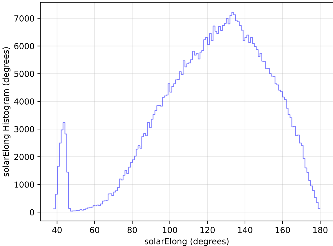
ddf_loaded_fl8_v3.4_10yrs All sky r band: solarElong Histogram
