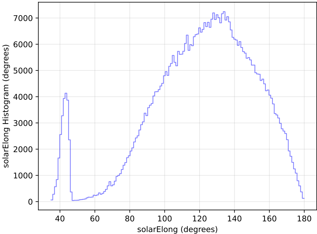
ddf_loaded_fl8_v3.4_10yrs All sky i band: solarElong Histogram
