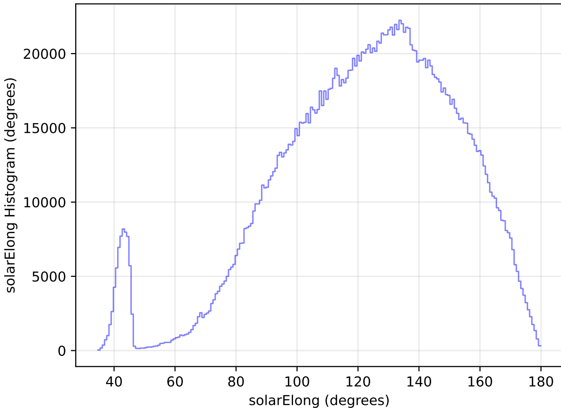
ddf_loaded_fl8_v3.4_10yrs All sky all bands: solarElong Histogram
