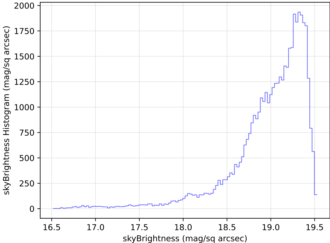
ddf_loaded_fl8_v3.4_10yrs Yr 1 z band: skyBrightness Histogram
