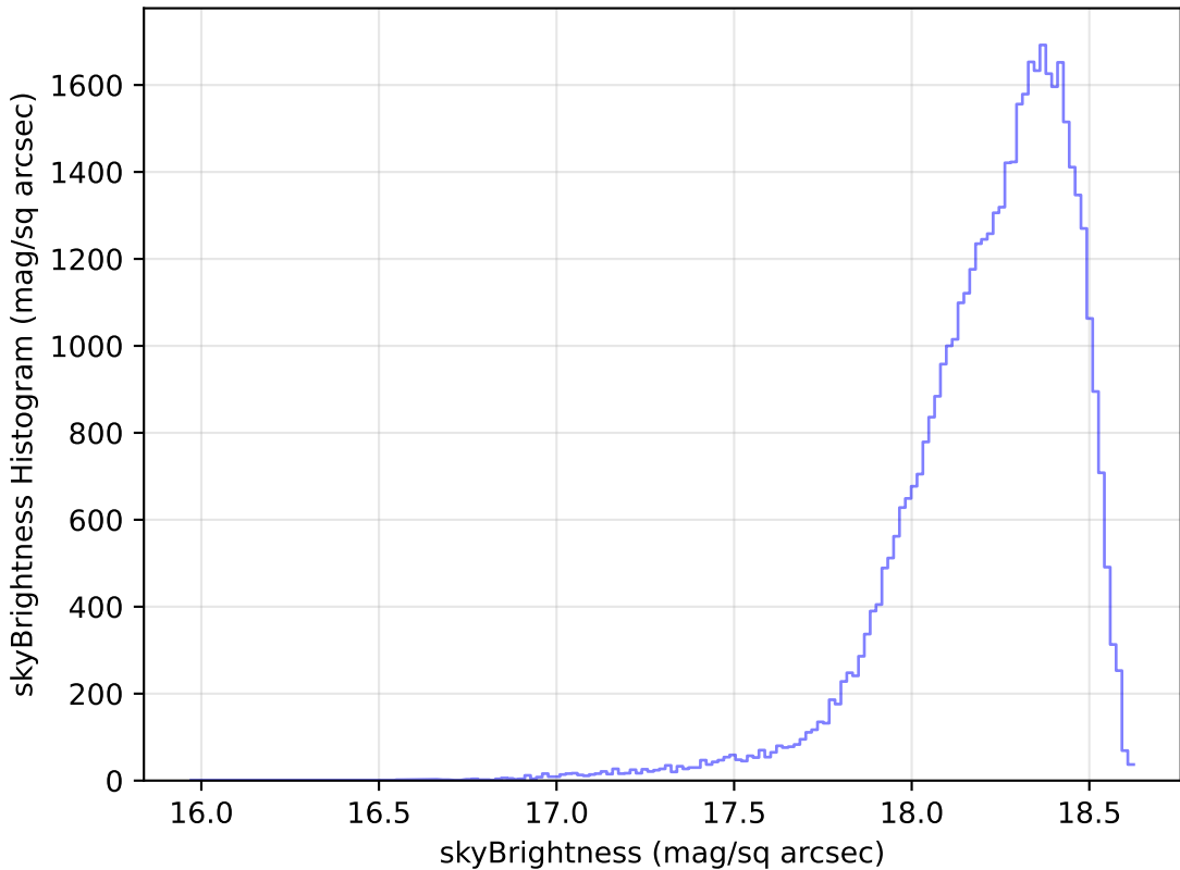
ddf_loaded_fl8_v3.4_10yrs Yr 1 y band: skyBrightness Histogram
