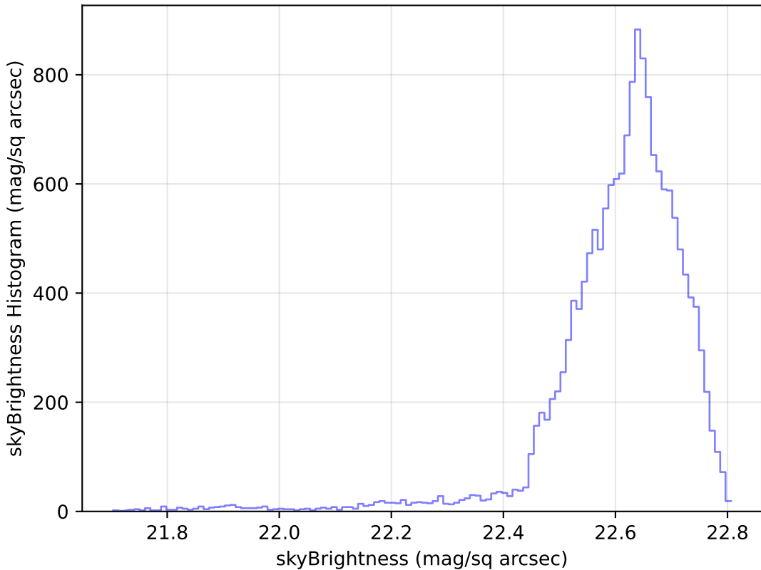
ddf_loaded_fl8_v3.4_10yrs Yr 1 u band: skyBrightness Histogram
