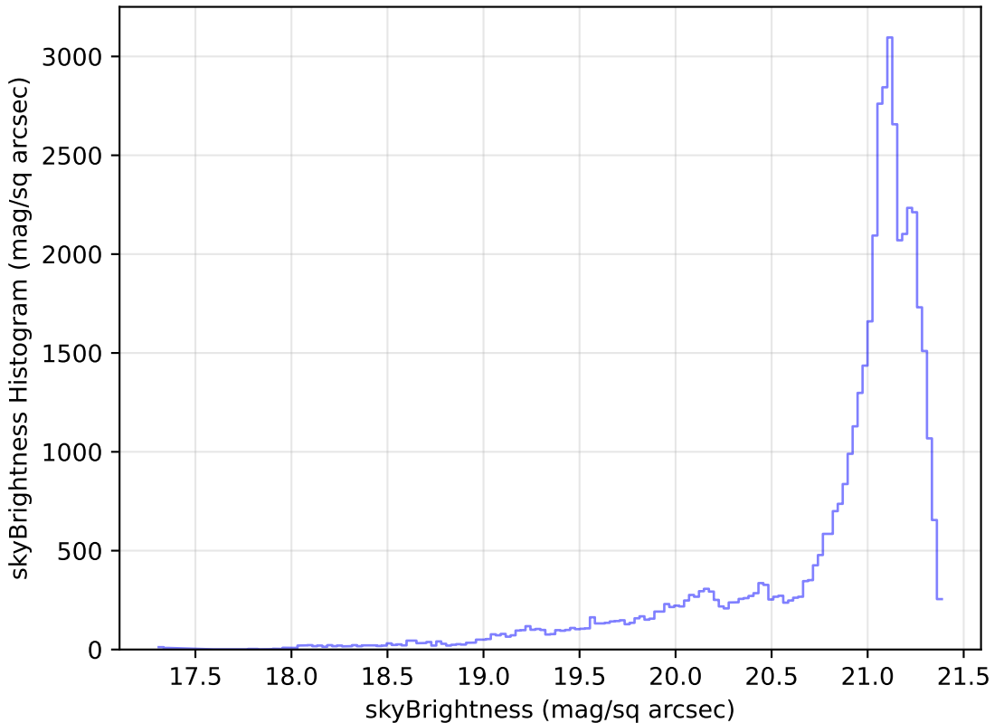
ddf_loaded_fl8_v3.4_10yrs Yr 1 r band: skyBrightness Histogram
